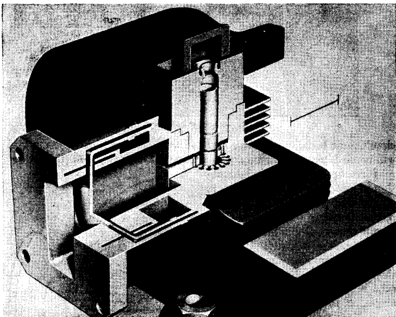
FIG. 5-5.—Waveguide output.
